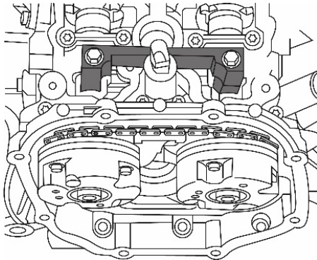
Camshaft Locking Tool, to be used as OEM T40070
