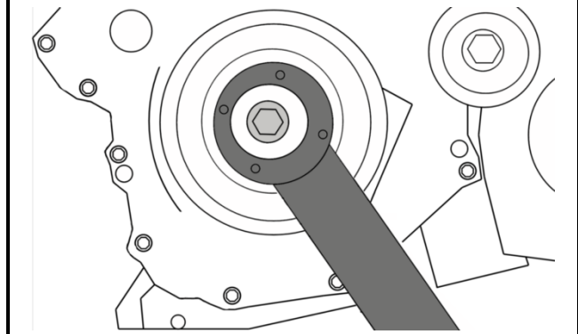
Crankshaft Pulley Holding Tool, to be used as OEM T10355
