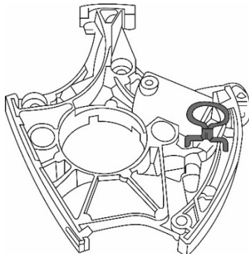
Chain Tensioner Locking Tool, to be used as OEM T40071
