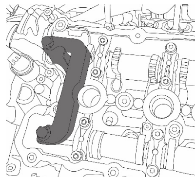
Camshaft Locking Tool, to be used as OEM T40133
